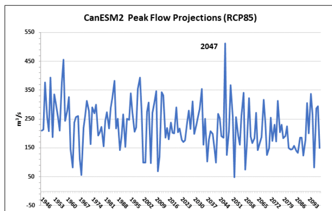
Figure 7 Projected peak annual flow of the Goat River based on the CanESM2 (RCP85) model. The 6-model ensemble RP for a flow threshold of 450\text{m}^3/\text{s} over the period 2036 – 2065 is 86 yrs. Excluding this single outlier from the 6-model average RP yields an average RP of 127 yrs for the 2036 – 2065 interval.
