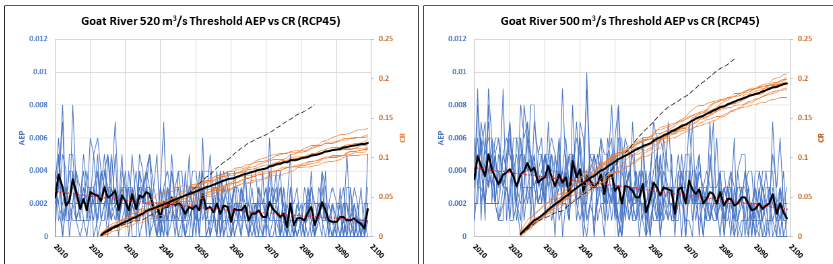
Figure B 4 Simulated Annual Exceedance Probability (AEP) and Cumulative Risk (CR) plots for Goat River flow thresholds of 520m³/s and 500 m³/s with RCP45. Orange curves show CR and blue curves show AEP. Heavy black curves show the average of 10 simulations. The thin dashed curve shows the CR based on the 6-member ensemble of PCIC Hydrologic models. Note scale change between pairs of plots.
