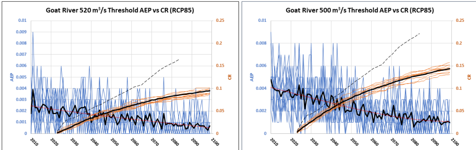
Figure B 1 Simulated Annual Exceedance Probability (AEP) and Cumulative Risk (CR) plots for Goat River flow thresholds of 520m³/s and 500 m³/s with RCP85. Orange curves show CR and blue curves show AEP. Heavy black curves show the average of 10 simulations. The thin dashed curve shows the CR based on the 6-member ensemble of PCIC Hydrologic models. Note scale change between pairs of plots.
