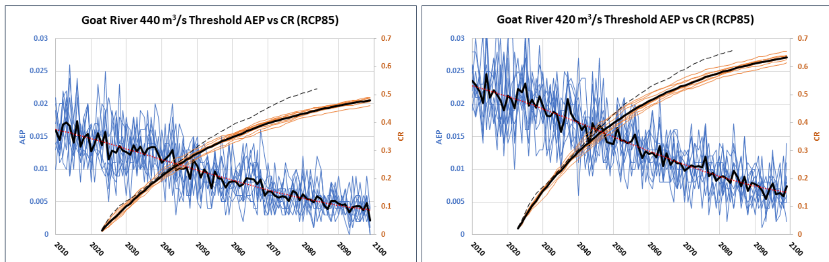
Figure B 3 Simulated Annual Exceedance Probability (AEP) and Cumulative Risk (CR) plots for Goat River flow thresholds of 440m³/s and 420 m³/s with RCP85. Orange curves show CR and blue curves show AEP. Heavy black curves show the average of 10 simulations. The thin dashed curve shows the CR based on the 6-member ensemble of PCIC Hydrologic models. Note scale change between pairs of plots.
