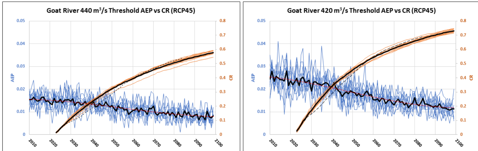
Figure B 6 Simulated Annual Exceedance Probability (AEP) and Cumulative Risk (CR) plots for Goat River flow thresholds of 440m³/s and 420 m³/s with RCP45. Orange curves show CR and blue curves show AEP. Heavy black curves show the average of 10 simulations. The thin dashed curve shows the CR based on the 6-member ensemble of PCIC Hydrologic models. Note scale change between pairs of plots.
