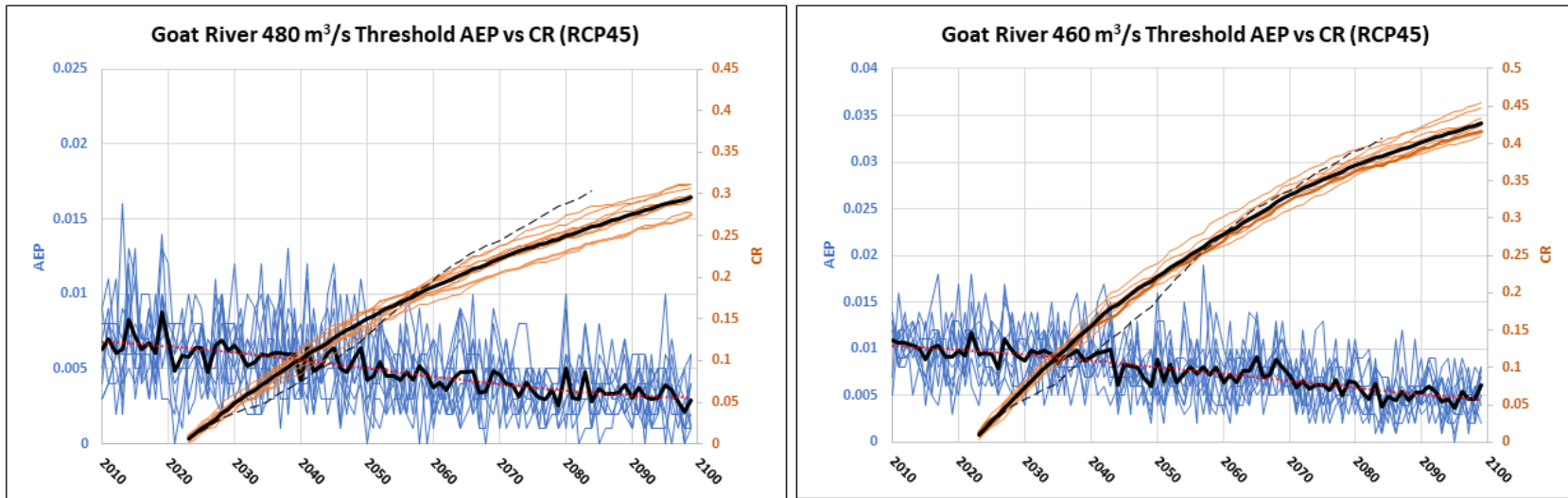
Figure B 5 Simulated Annual Exceedance Probability (AEP) and Cumulative Risk (CR) plots for Goat River flow thresholds of 480m³/s and 460 m³/s with RCP45. Orange curves show CR and blue curves show AEP. Heavy black curves show the average of 10 simulations. The thin dashed curve shows the CR based on the 6-member ensemble of PCIC Hydrologic models. Note scale change between pairs of plots.
