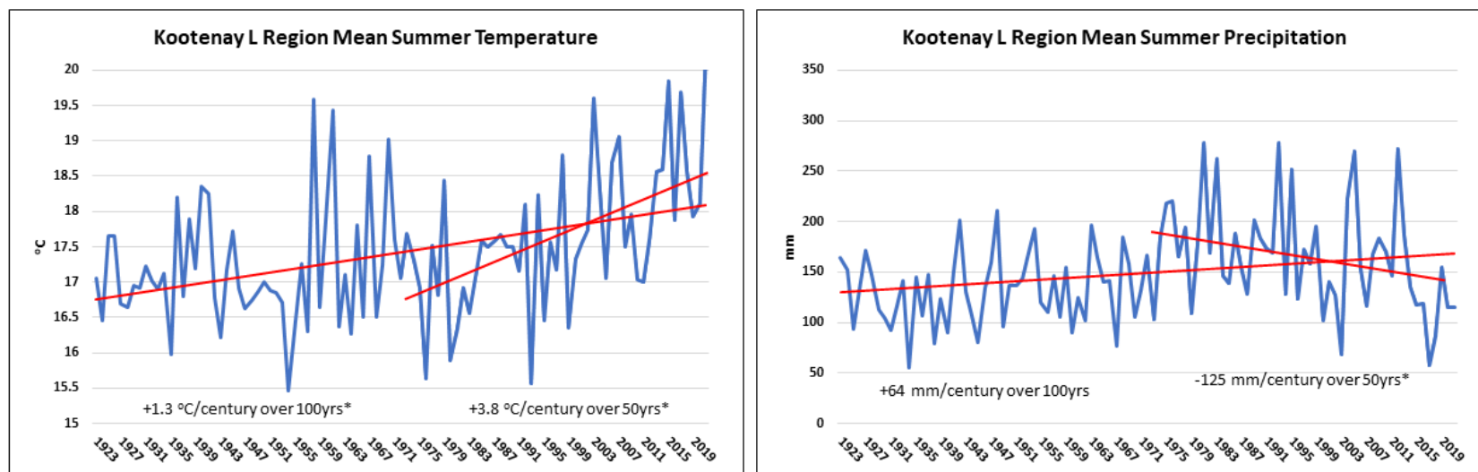
Figure A 7 a) Kootenay Lake region mean summer temperature over the last 100 years with 100-year trend and trend over the last 50 years. b) Kootenay Lake region mean summer precipitation over the last 100 years with 100-year trend and trend over the last 50 years. Trends that are statistically significant at the 95% confidence are identifies with *.
