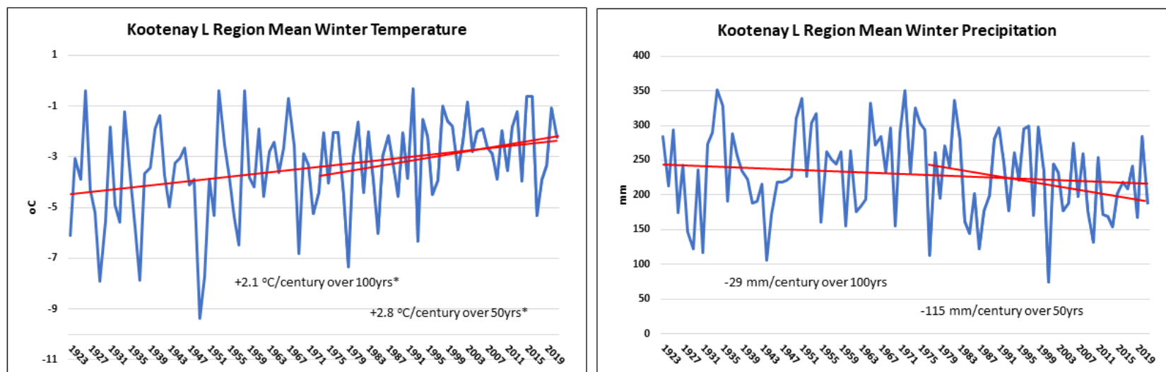
Figure A 5 a) Kootenay Lake region mean winter temperature over the last 100 years with 100-year trend and trend over the last 50 years. b) Kootenay Lake region mean winter precipitation over the last 100 years with 100-year trend and trend over the last 50 years. Trends that are statistically significant at the 95% confidence are identifies with *.
