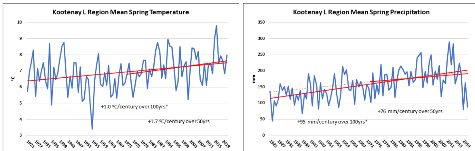
Figure A 6 a) Kootenay Lake region mean spring temperature over the last 100 years with 100-year trend and trend over the last 50 years. b) Kootenay Lake region mean spring precipitation over the last 100 years with 100-year trend and trend over the last 50 years. Trends that are statistically significant at the 95% confidence are identifies with *.
