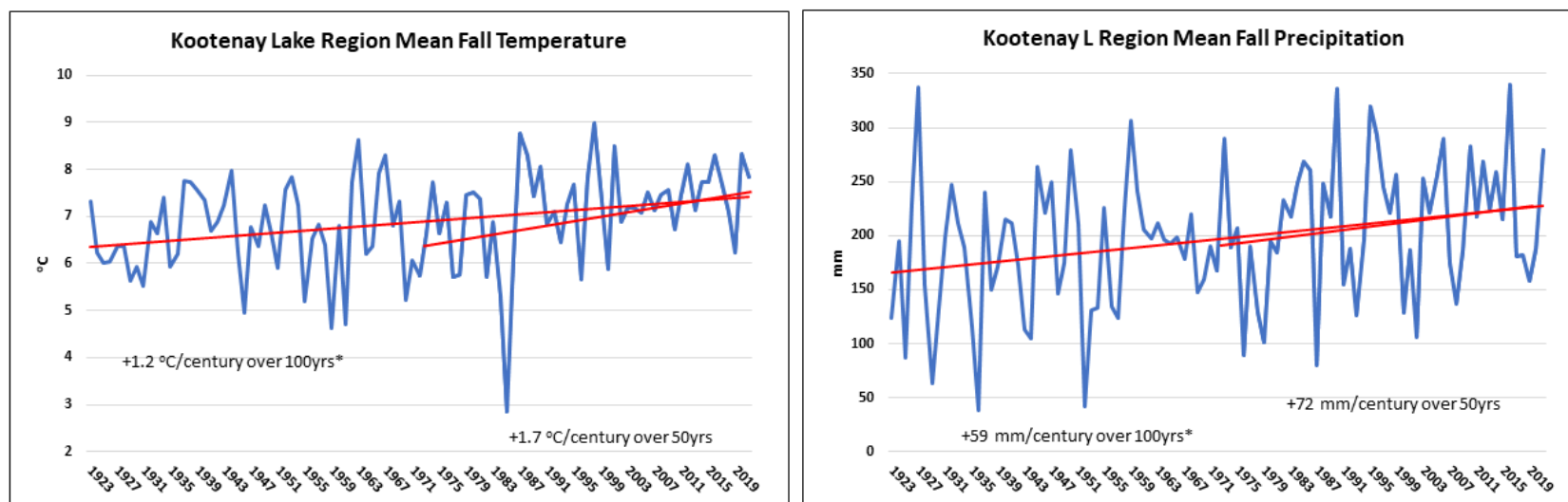
Figure A 8 a) Kootenay Lake region mean fall temperature over the last 100 years with 100-year trend and trend over the last 50 years. b) Kootenay Lake region mean fall precipitation over the last 100 years with 100-year trend and trend over the last 50 years. Trends that are statistically significant at the 95% confidence are identifies with *.
