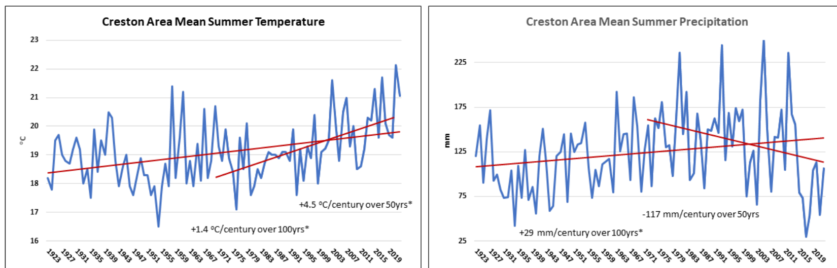
Figure A 3 a) Creston area mean summer temperature over the last 100 years with 100-year trend and trend over the last 50 years. b) Creston area mean summer precipitation over the last 100 years with 100-year trend and trend over the last 50 years. Trends that are statistically significant at the 95% confidence are identifies with *.
