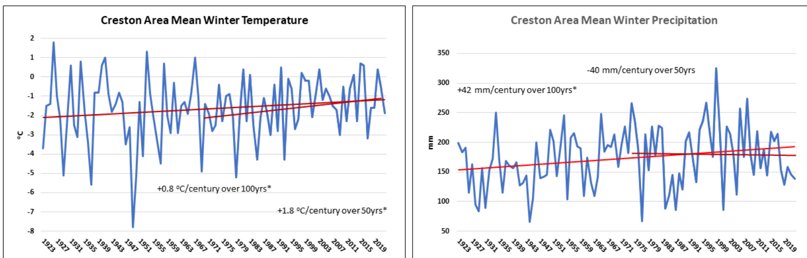
Figure A 1 a) Creston area mean winter temperature over the last 100 years with 100-year trend and trend over the last 50 years. b) Creston area mean winter precipitation over the last 100 years with 100-year trend and trend over the last 50 years. Trends that are statistically significant at the 95% confidence are identified with *.
