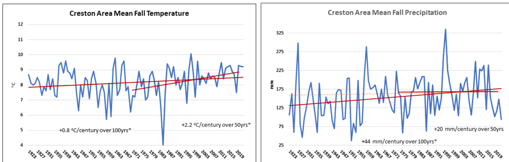
Figure A 4 a) Creston area mean fall temperature over the last 100 years with 100-year trend and trend over the last 50 years. b) Creston area mean fall precipitation over the last 100 years with 100-year trend and trend over the last 50 years. Trends that are statistically significant at the 95% confidence are identified with *.
