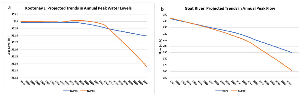
Figure 16 General projected trends for peak annual Kootenay Lake levels. Figure 16b. General projected trends for peak annual Goat River flow. Blue curves represent RCP45 model projections. Orange curves represent RCP85 model projections.
