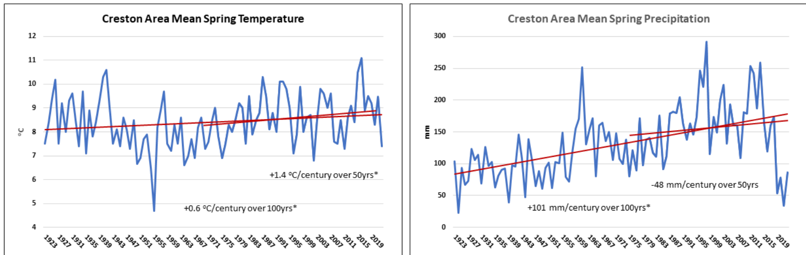
Figure A 2 a) Creston area mean spring temperature over the last 100 years with 100-year trend and trend over the last 50 years. b) Creston area mean spring precipitation over the last 100 years with 100-year trend and trend over the last 50 years. Trends that are statistically significant at the 95% confidence are identifies with *.
